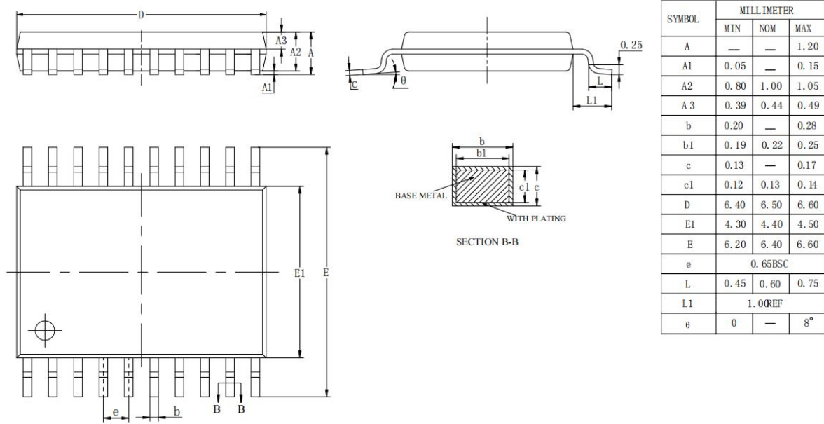
Figure 4-1 AW314A Package
