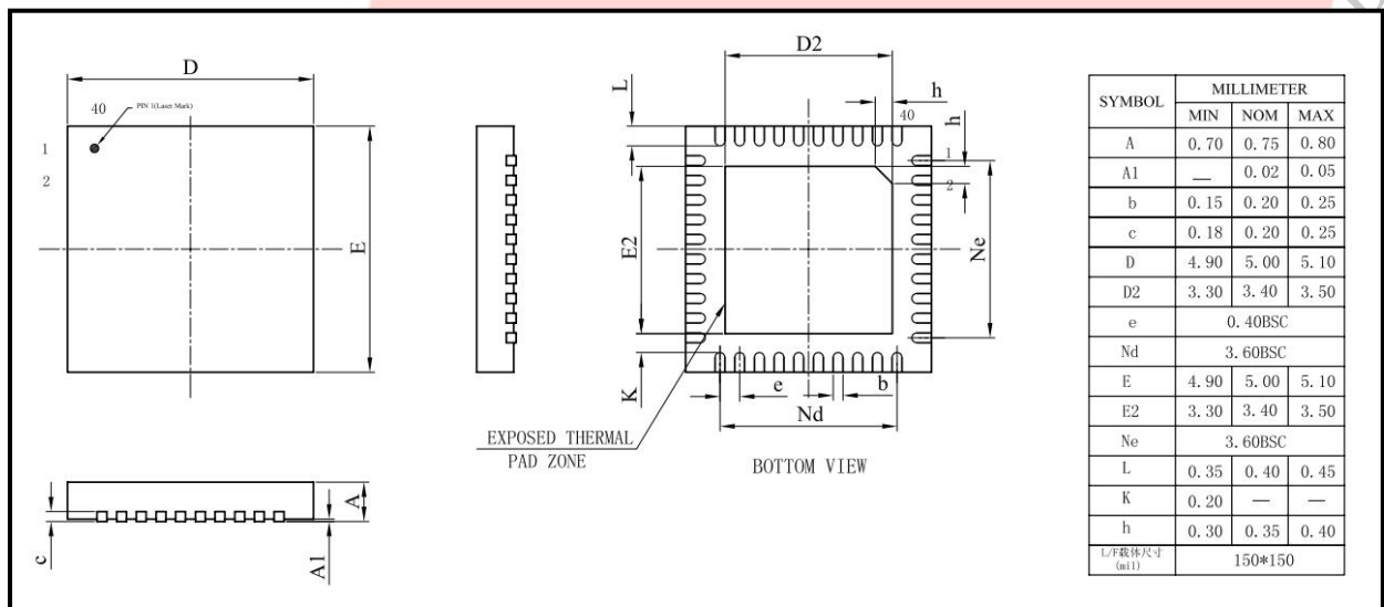
Figure 3-1 AC7913A6_QFN40 Package
