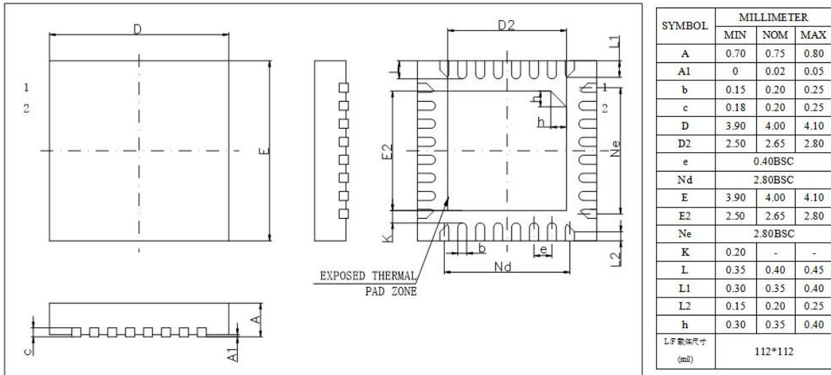
Figure 4-1 AW306A Package
