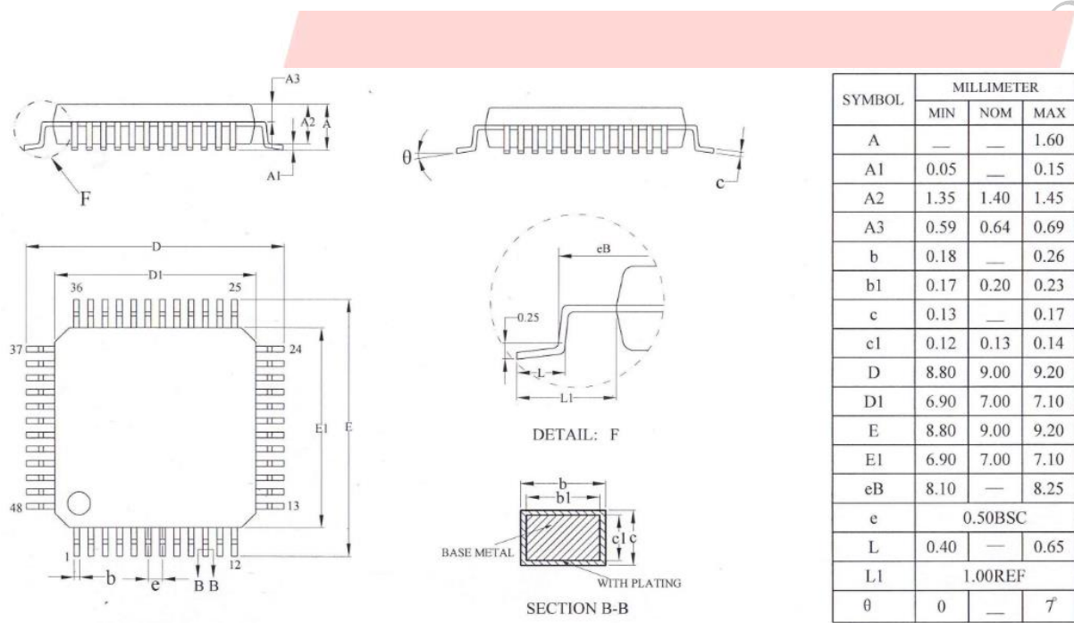
Figure 3-1. AC6951B_LQFP48 Package
