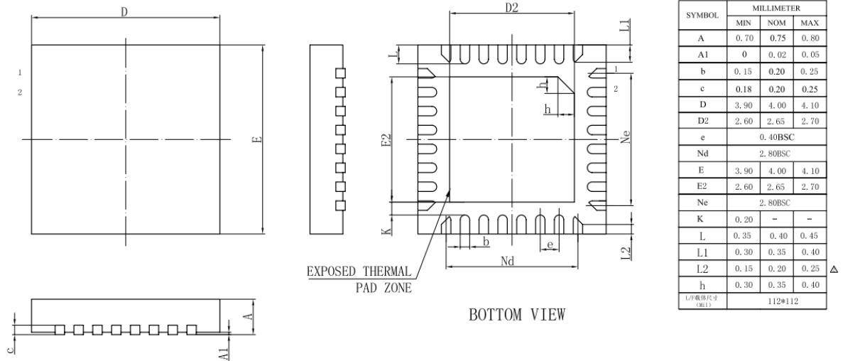
Figure 3-1 AC6956C Package
