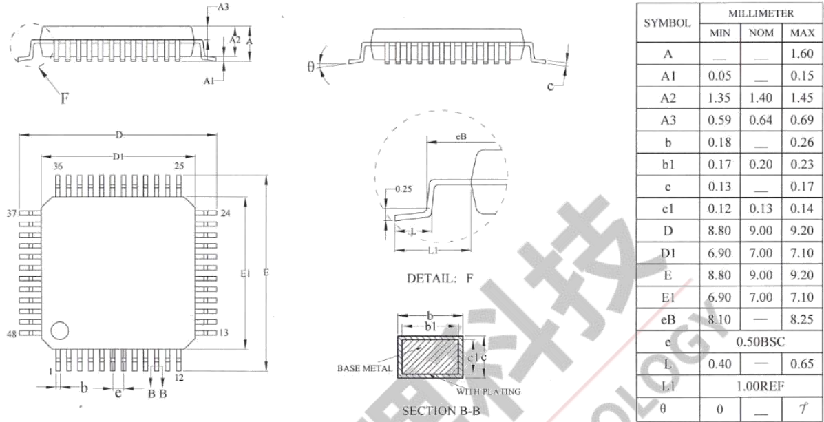
Figure 4-1 AD161A Package
