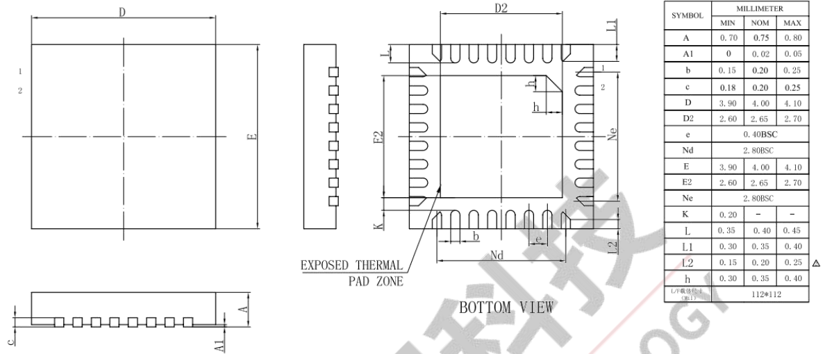
Figure 4-1 AD176A Package
