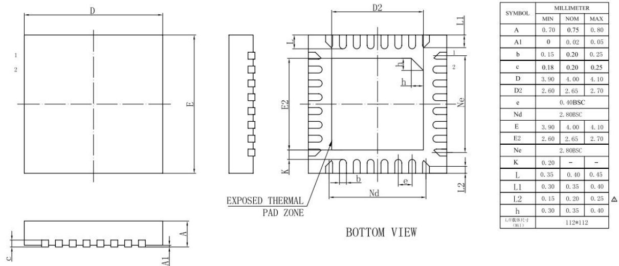
Figure 4-1 AC7066M Package
