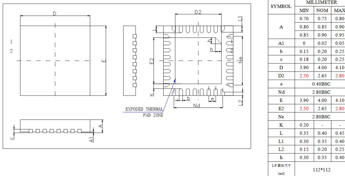
Figure 4-1 AC7066A Package
