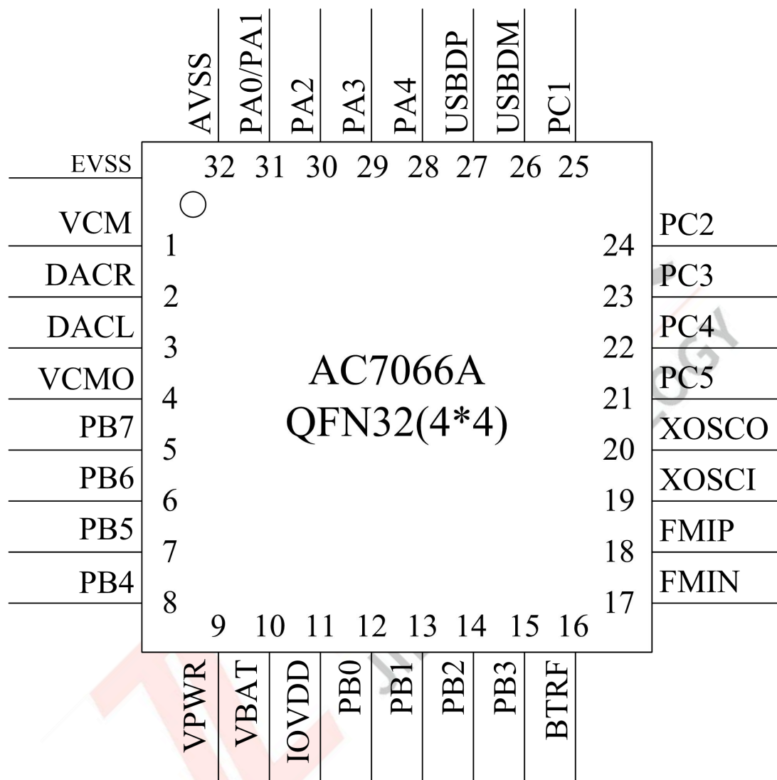
Figure 2-1 AC7066A Pin Assignment
