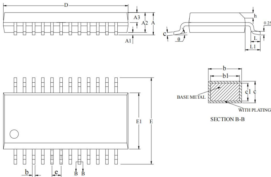
Figure 4-1 AC7065D Package
