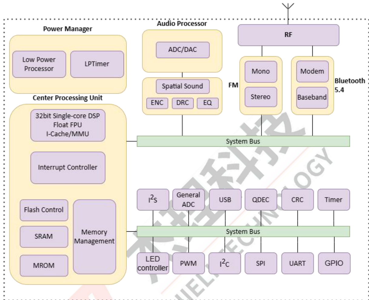
Figure 1-1 AC7065D Block Diagram
