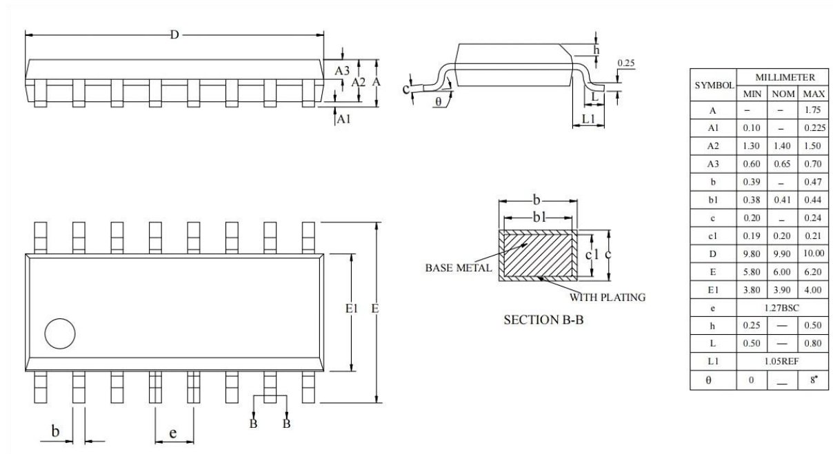
Figure 4-1 AW312B Package
