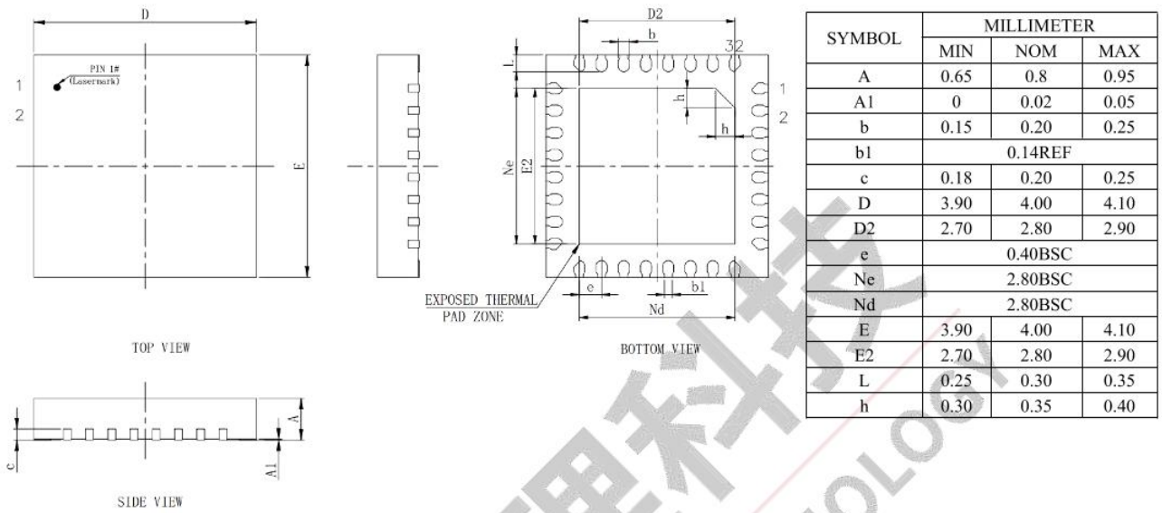
Figure 4-1 AC7076A Package
