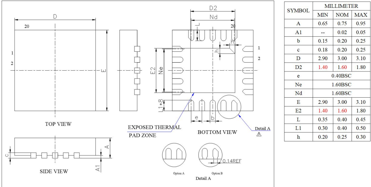
Figure 4-1 AW309A Package
