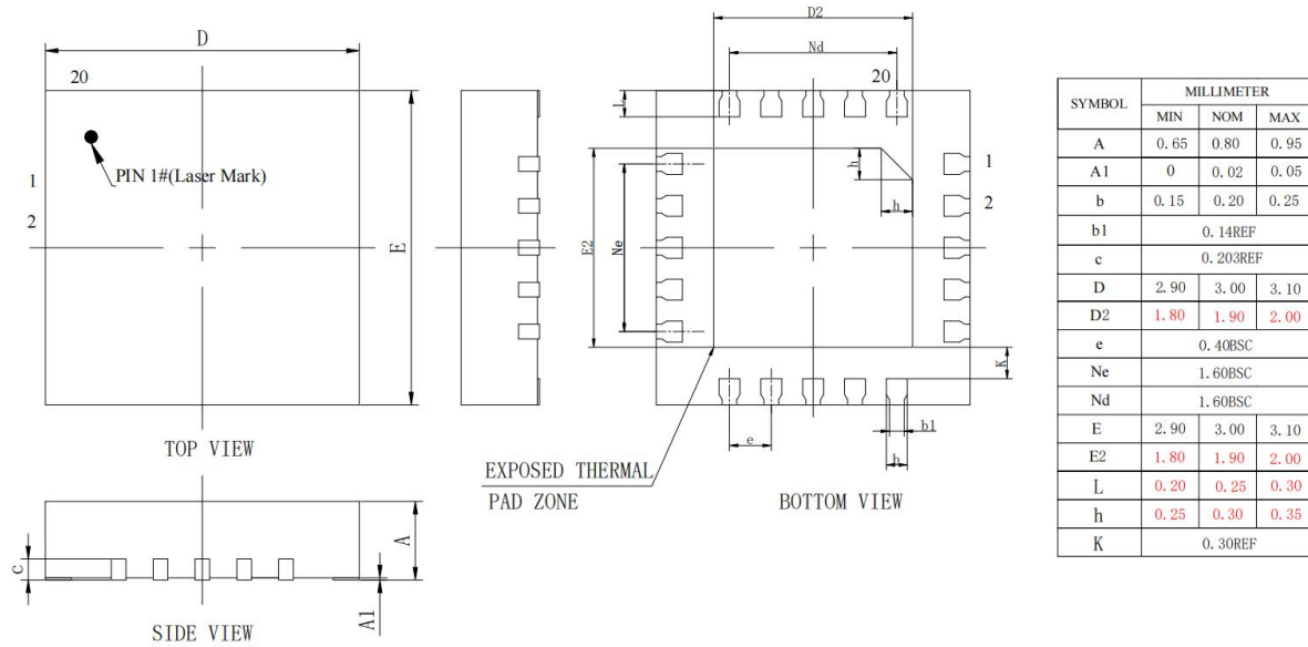
Figure 4-1 AC7103D Package
