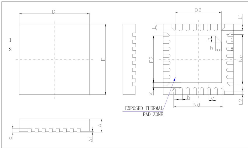
Figure 4-1 AC7106F Package
