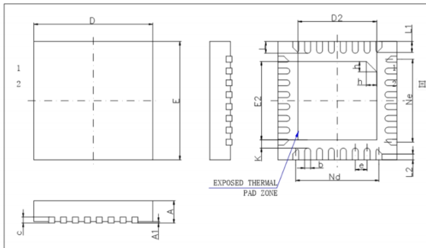
Figure 4-1 AC2106C Package
