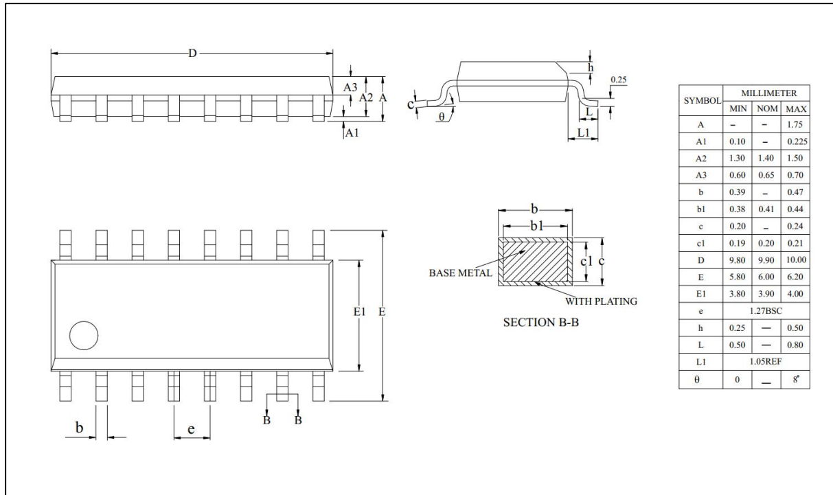
Figure 4-1 AW332A Package
