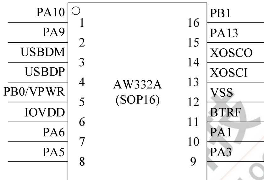
Figure 2-1 AW332A Pin Assignment
