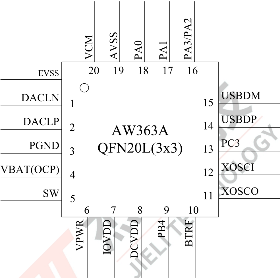
Figure 2-1 AW363A Pin Assignment
