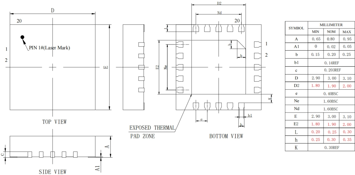
Figure 4-1 AW363A Package
