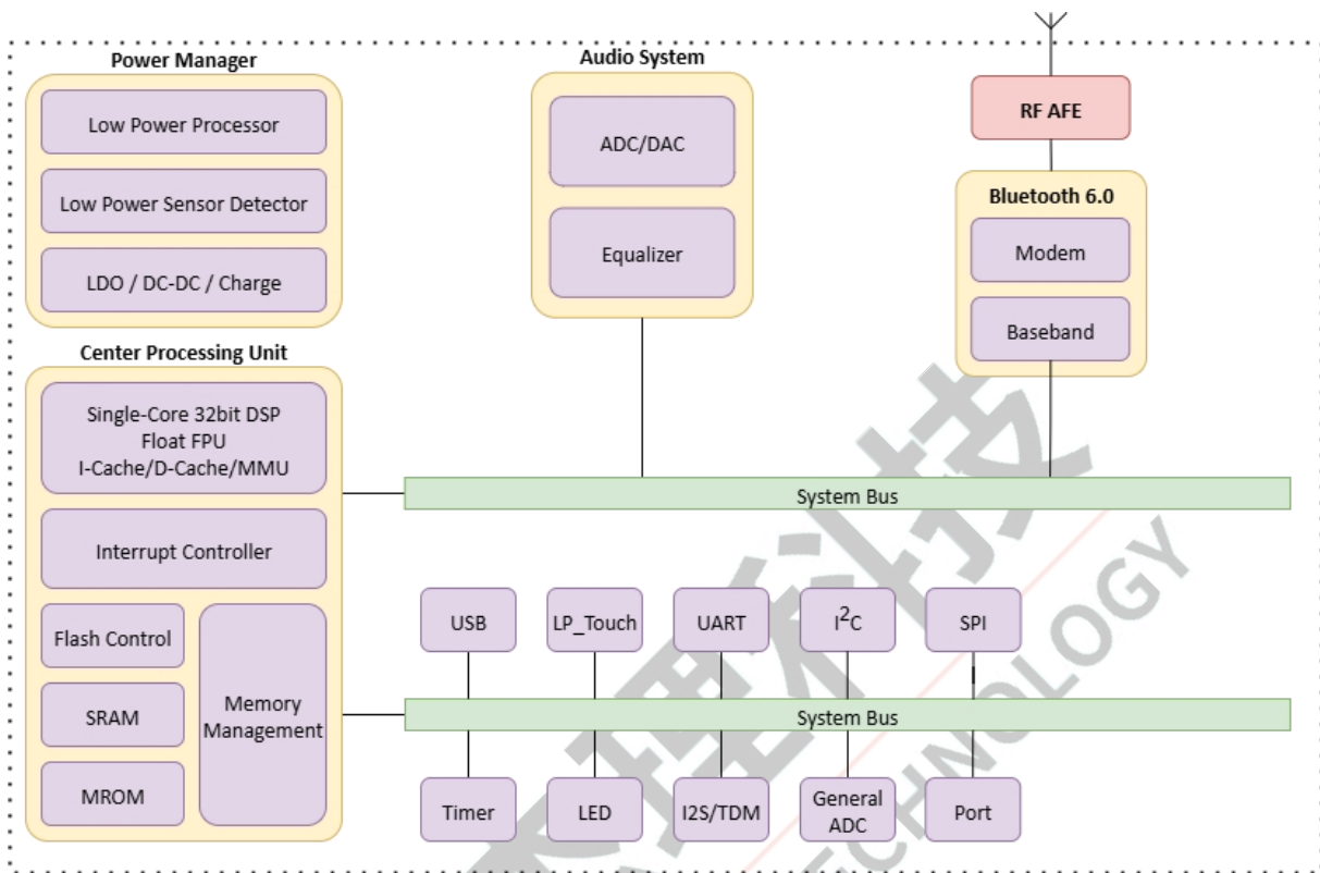
Figure 1-1 AW363A Block Diagram
